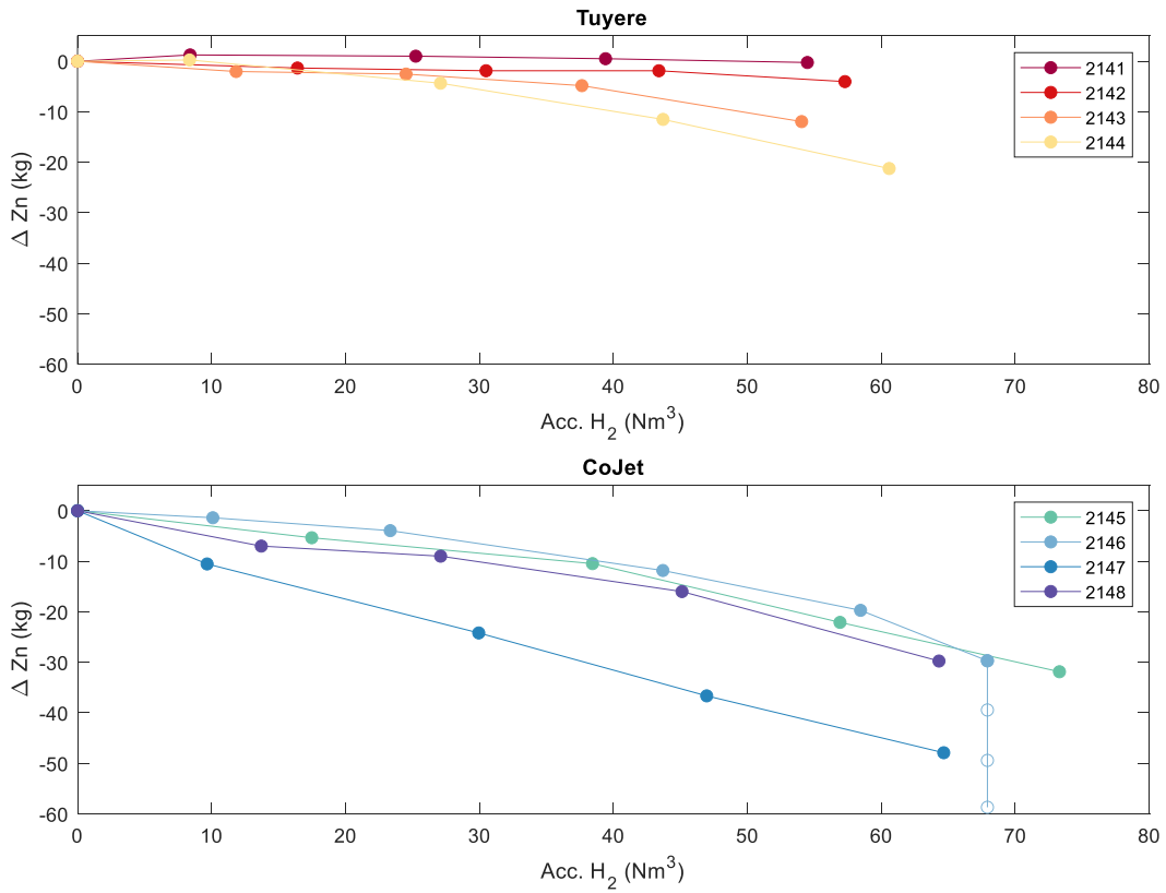
Figure 1. Change of zinc content (in kg) in the slag as a function of accumulated injected H 2 (in Nm 3 ).
